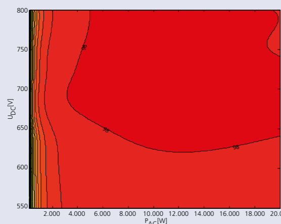
3D-Wirkungsgraddiagramm blueplanet 20.0 TL3 INT
